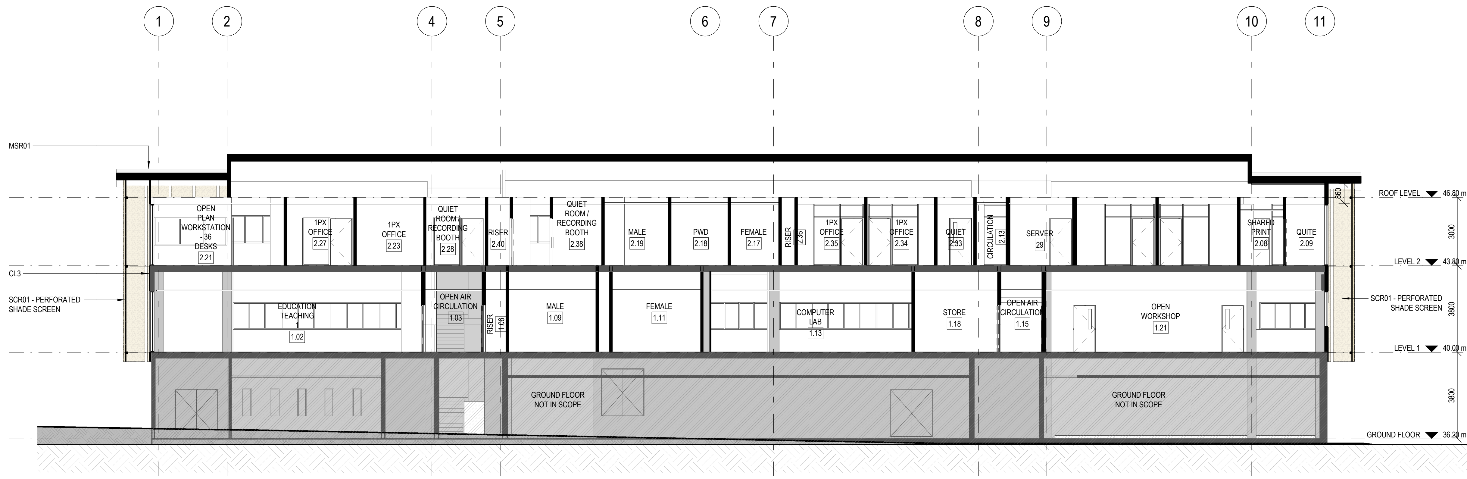
3 LONGITUDINAL SECTION - PROPOSED 1 : 100
