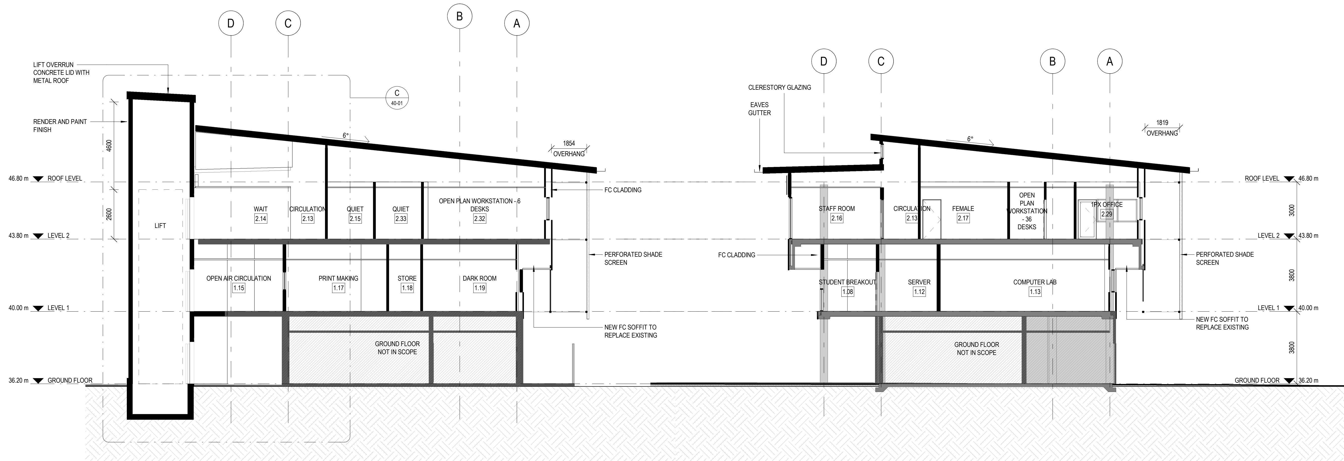
1 TRANSVERSAL SECTION 1 - PROPOSED 1 : 100
